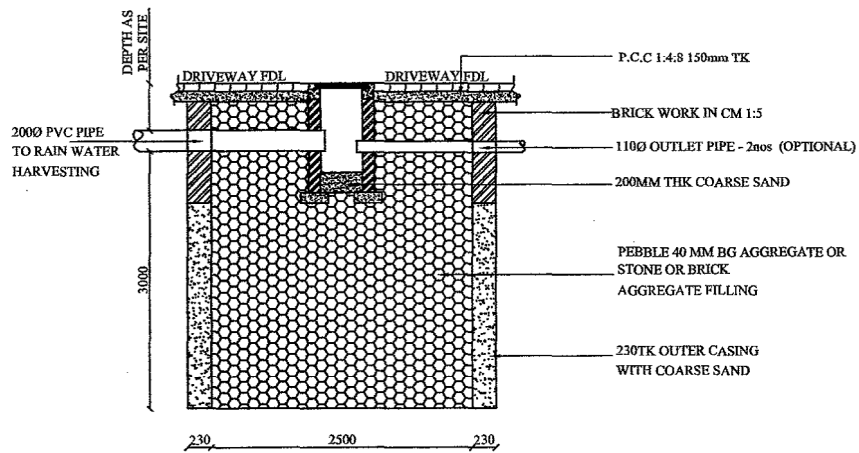
SOAKPIT DETAILS
